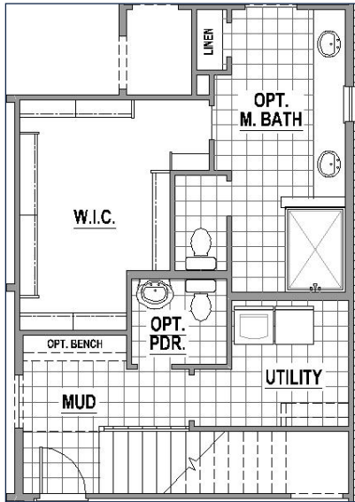
Optional 2nd Floor, Optional Main Bath Layout & Optional Powder Bath
