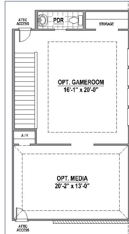
Optional Game Room and Media Room (+727 SF)
