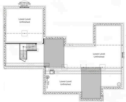
Lower Level
