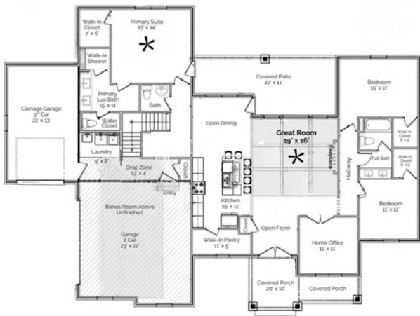
Main Level
