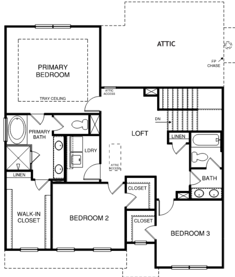
SECOND FLOOR
