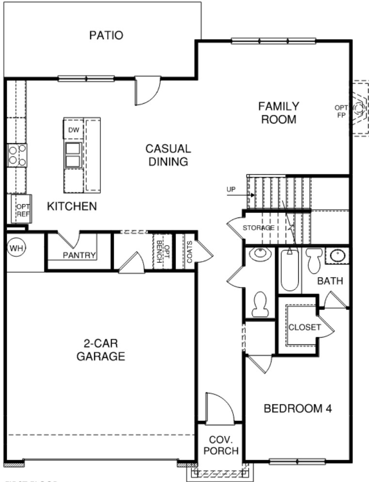
FIRST FLOOR
