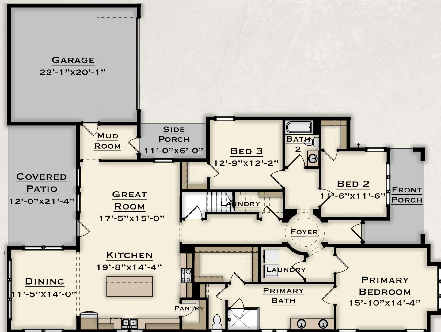
Main Level
