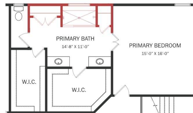
Second Floor shown with Optional Euro Shower
