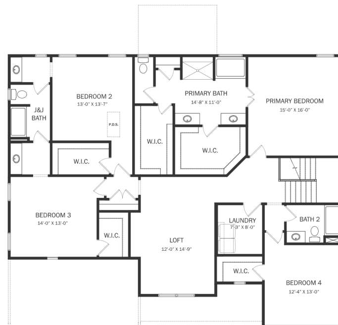
Included Second Floor
