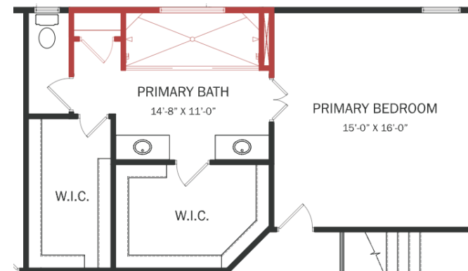
Second Floor shown with Optional Ultimate Layout
