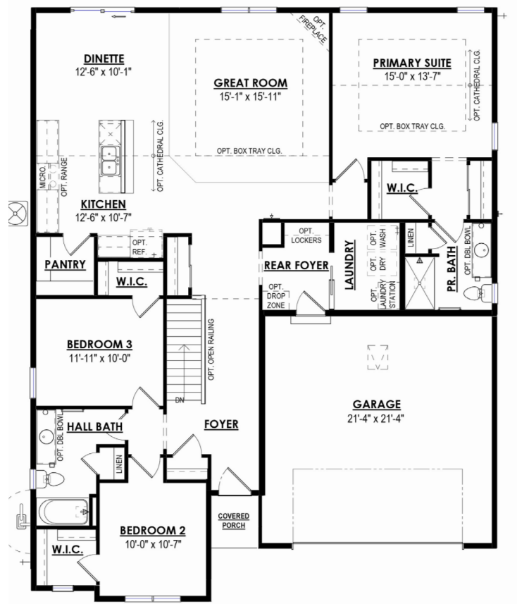
1st FLOOR 1,808 Sq. Ft.
