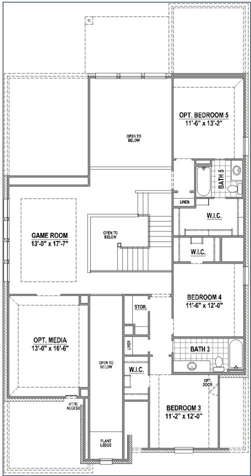
Optional Media Room, Bedroom 5 & Bath 5 (+593 SF)
