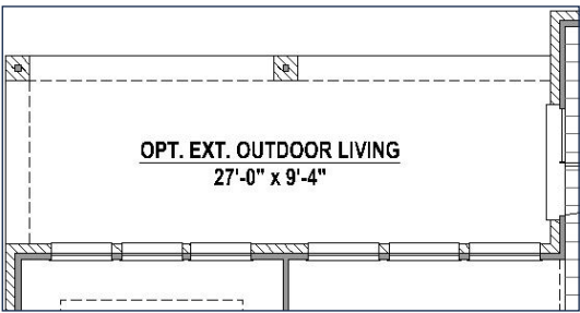
Optional Extended Outdoor Living (+124 SF)
