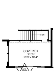
OPT. GARDEN LEVEL COVERED DECK
