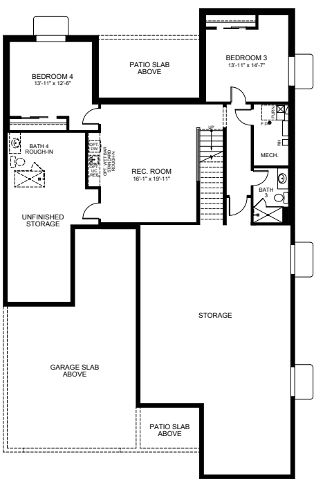
OPT. ENLARGED BASEMENT PLAN
