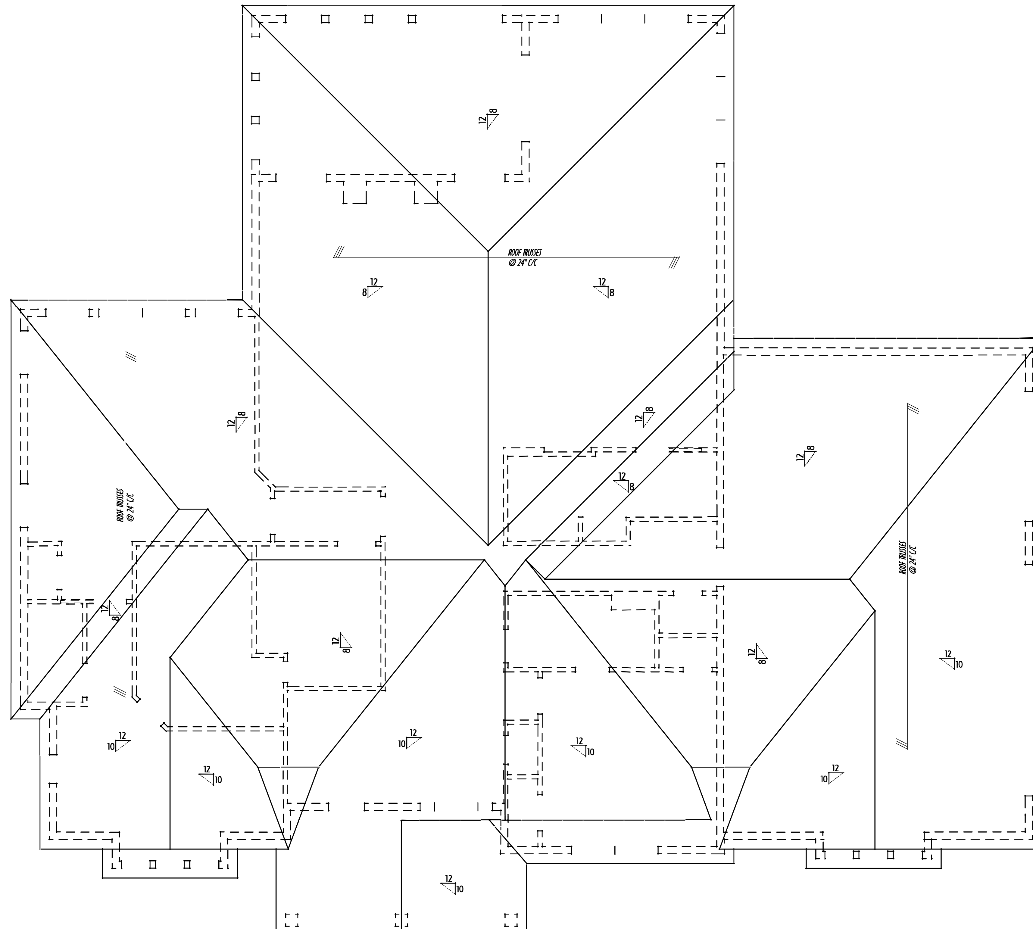
PRELIMINARY ROOF FRAMING LAYOUT
