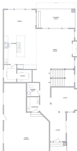
Main Floor
