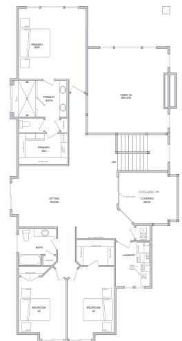
Upper Floor
