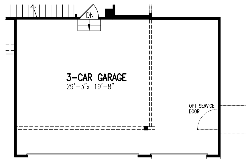
Opt 3-Car Garage Based on Elevation A
