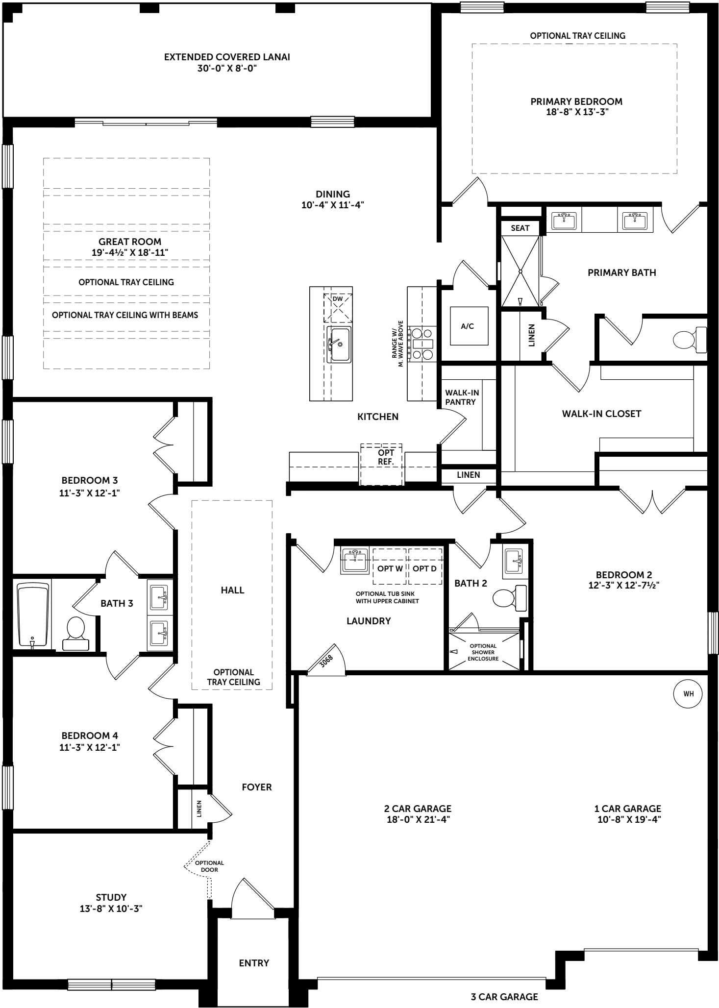
ELEVATION A 9' 4" CEILING
