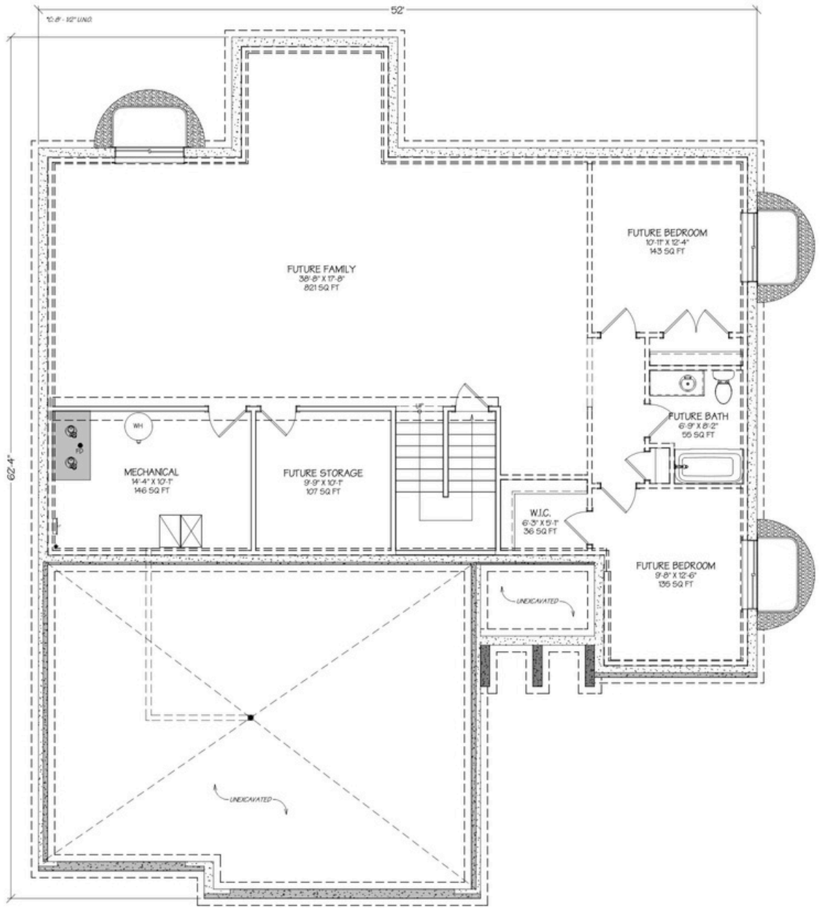
Sienna 3.0 - Base Plan - Lower Floor - 1,750 sq ft
