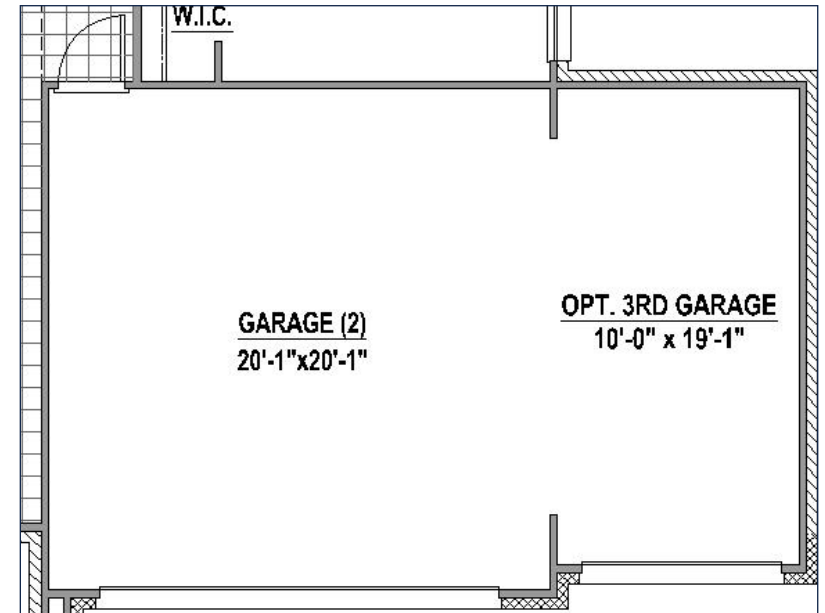
Optional 3rd Car Garage
