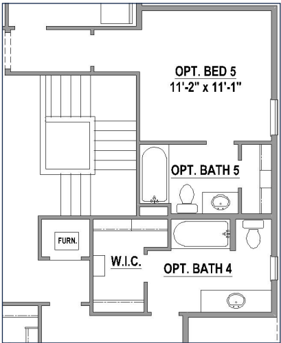
Optional Bed 5 w/Baths 4 & 5 (+268 SF)
