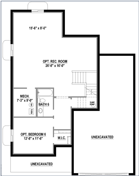
Optional Rec Room w/Bed 6 & Bath 6 (+1,036 SF)
