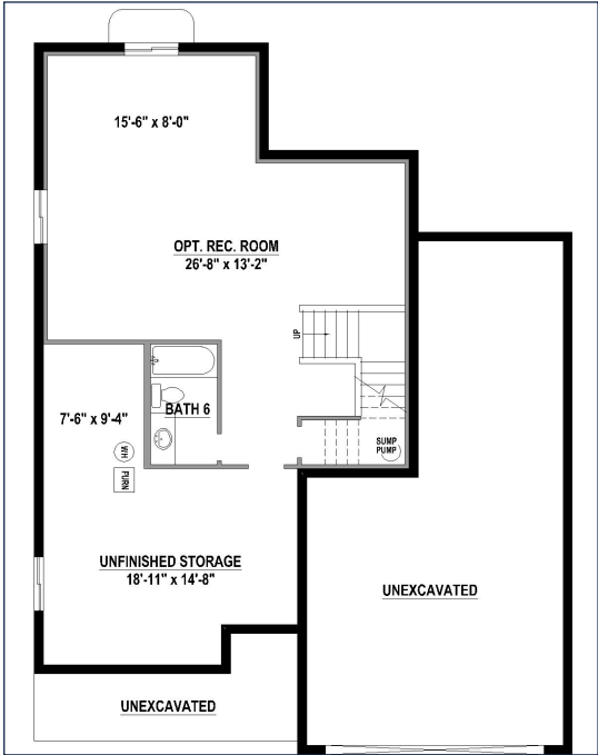
Optional Rec Room w/Bath (+746 SF)
