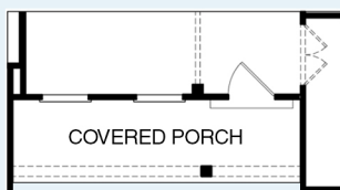
A1, A3, B PARTIAL FLOOR PLAN
