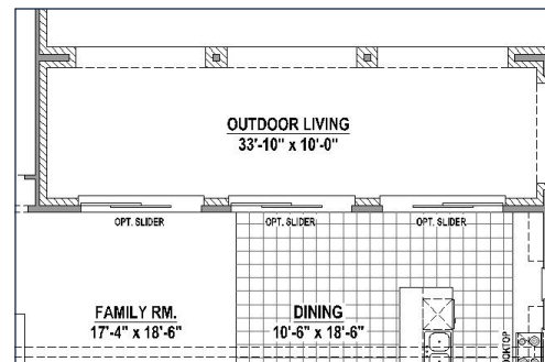
Multi-Sliding Doors at Outdoor Living
