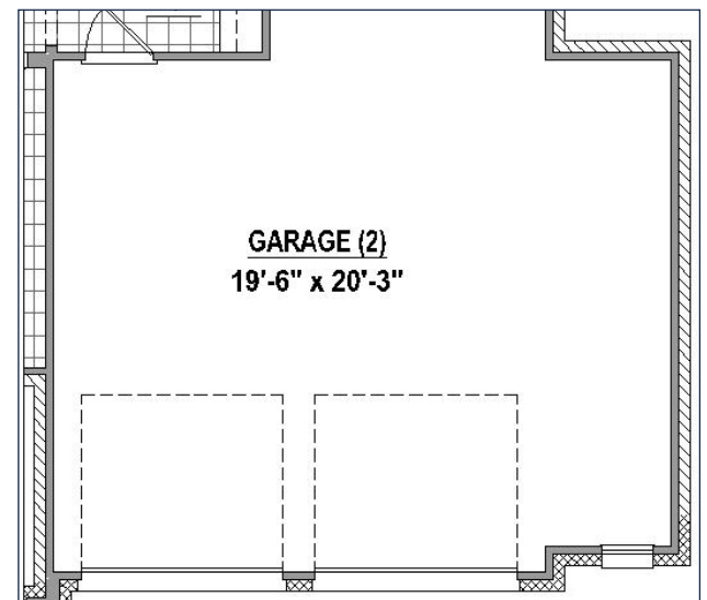
1/2 Car Garage
