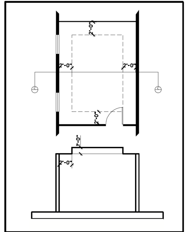
350-200-4205 (Box Ceiling)
