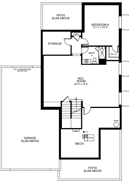
OPT. PARTIAL FINISHED BASEMENT
