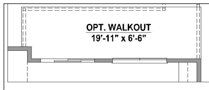
Walk-Out Basement
