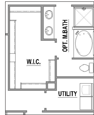
Alternate Main Bath Layout
