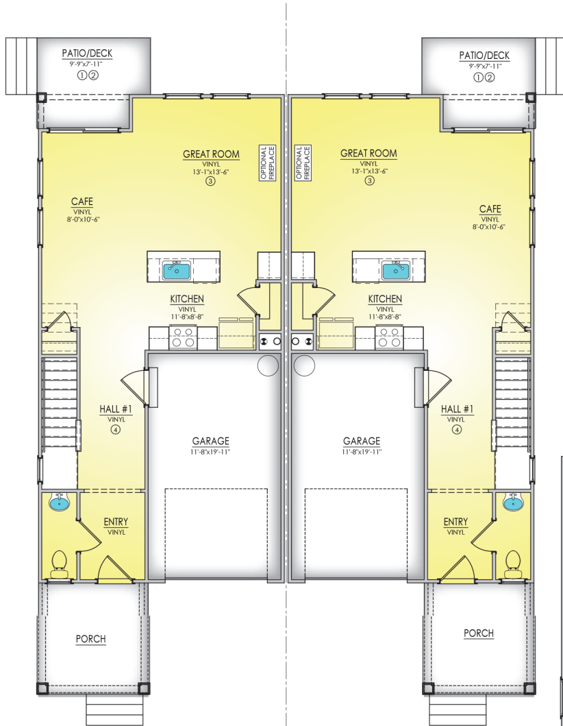
MAIN LEVEL - C
