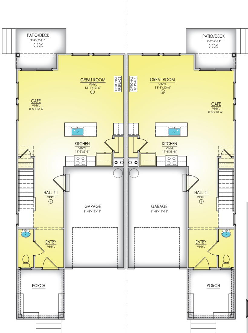
MAIN LEVEL - B
