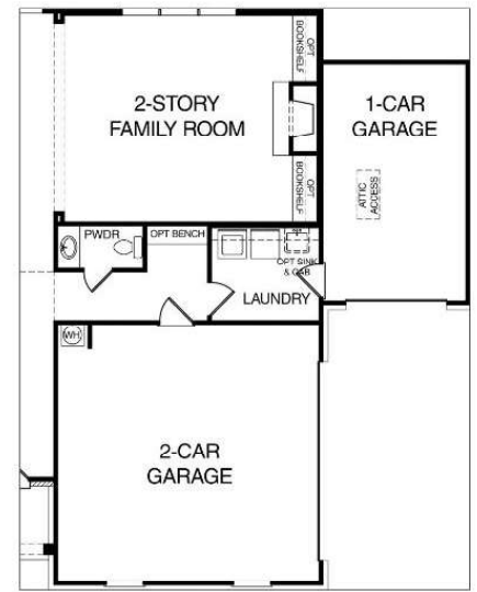
3-CAR SIDE ENTRY GARAGE
