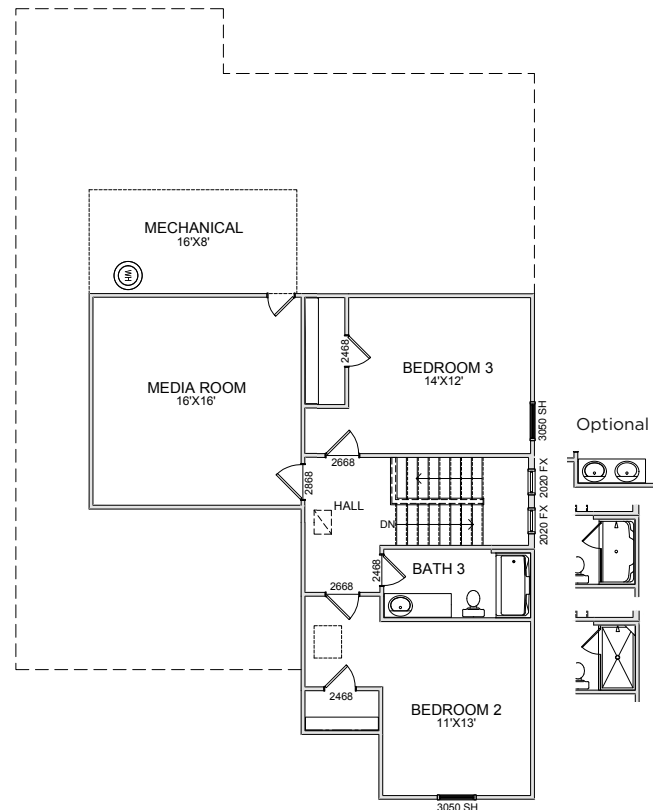
Second Floor
