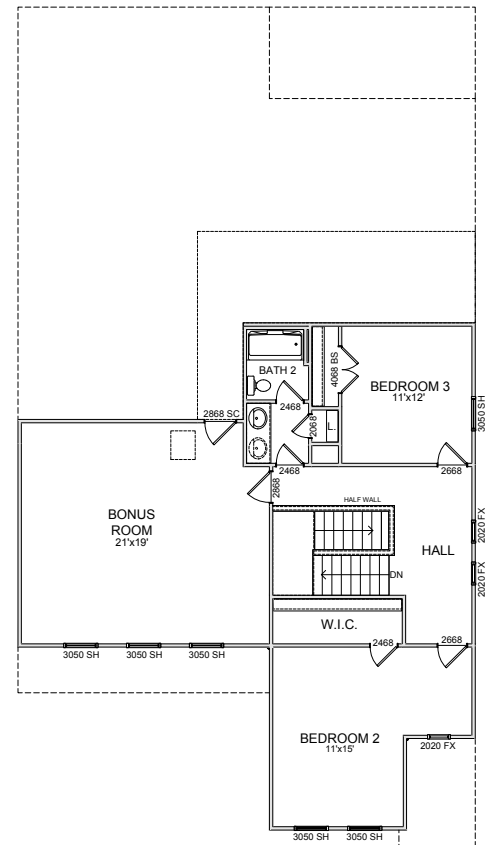
Second Floor
