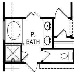
OPTIONAL PRIMARY BATH
