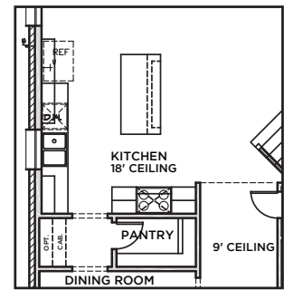
OPT. KITCHEN LAYOUT
