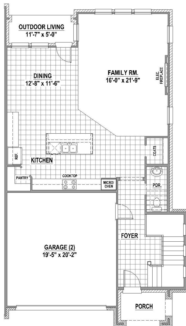
1 st Floor
