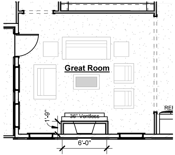
Great Room Fireplace Bump-In
