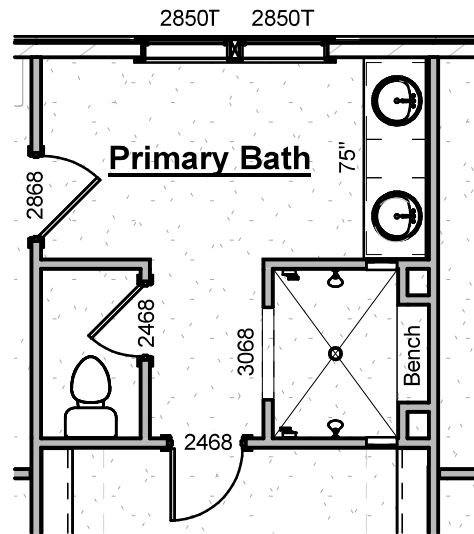
Primary Bath with Grotto Shower
