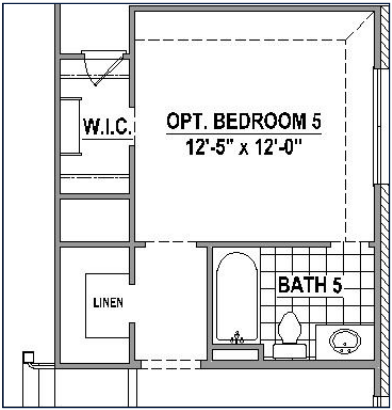
Optional Bedroom 5 with Bath 5 (+306 SF)
