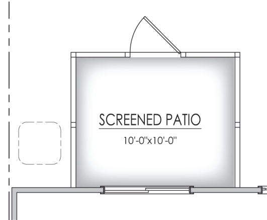
2 - OPTIONAL SCREENED PATIO
