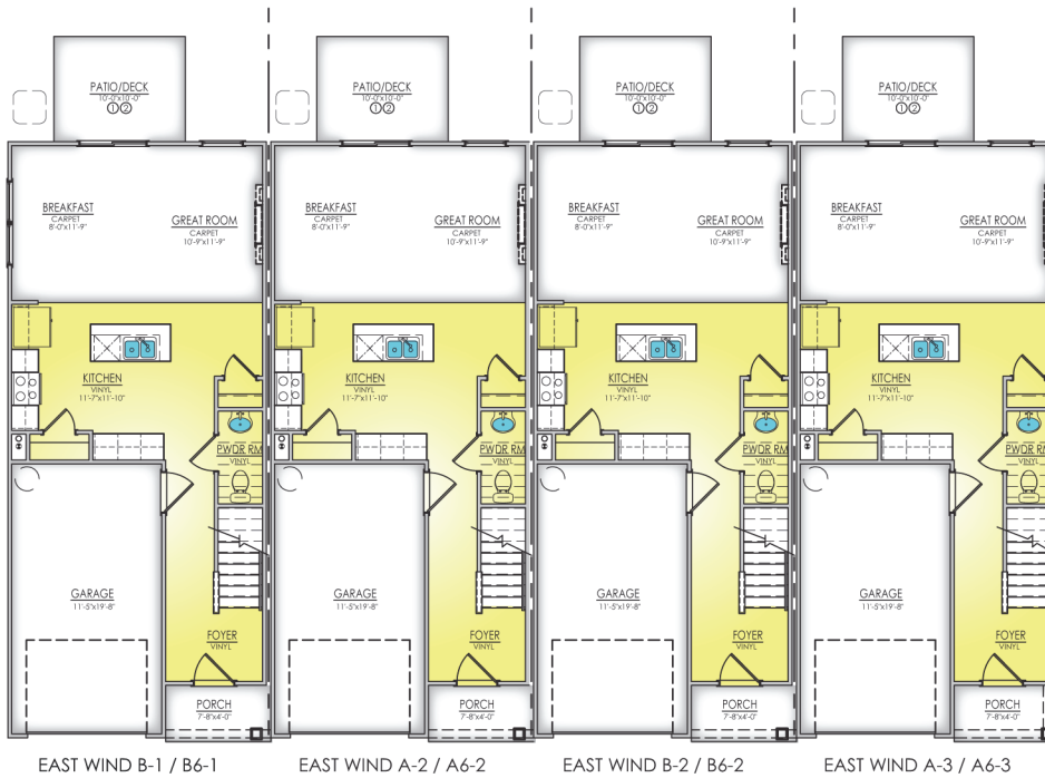
MAIN LEVEL - 4 UNITS
