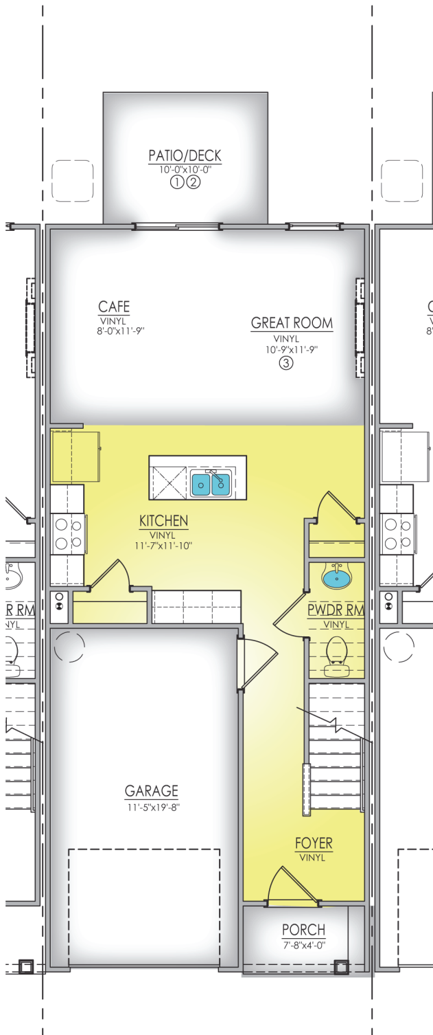
MAIN LEVEL - 5 UNITS
