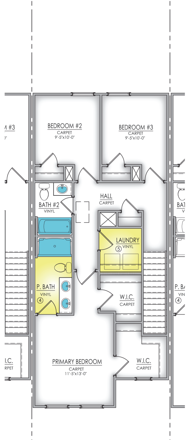
SECOND LEVEL - 5 UNITS
