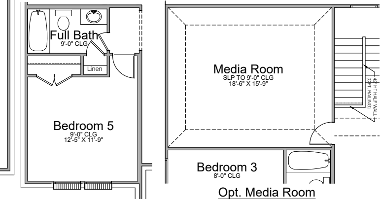
Opt. Bedroom 5 w/ Full Bath ilo Flex Room/Powder
