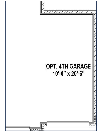
Optional 4th Car Garage
