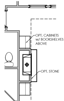
OPT. CABINETS @ FIREPLACE
