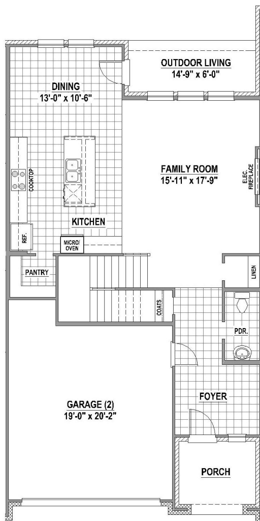
1 st Floor
