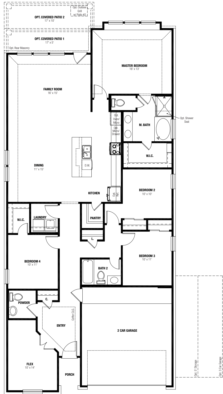
FIRST FLOOR
