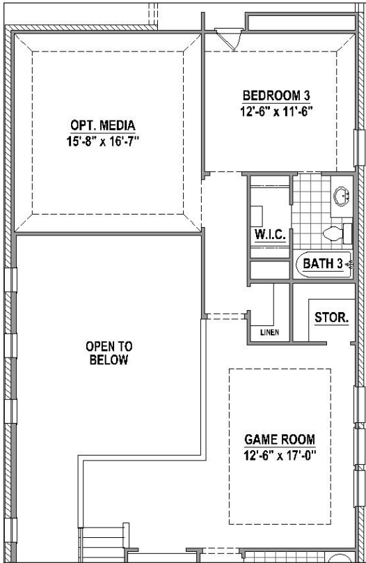
Media Room (+383 SF)
