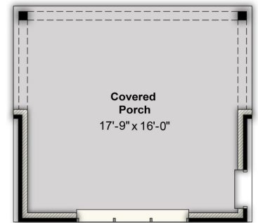
Opt. Extended Rear Covered Porch
