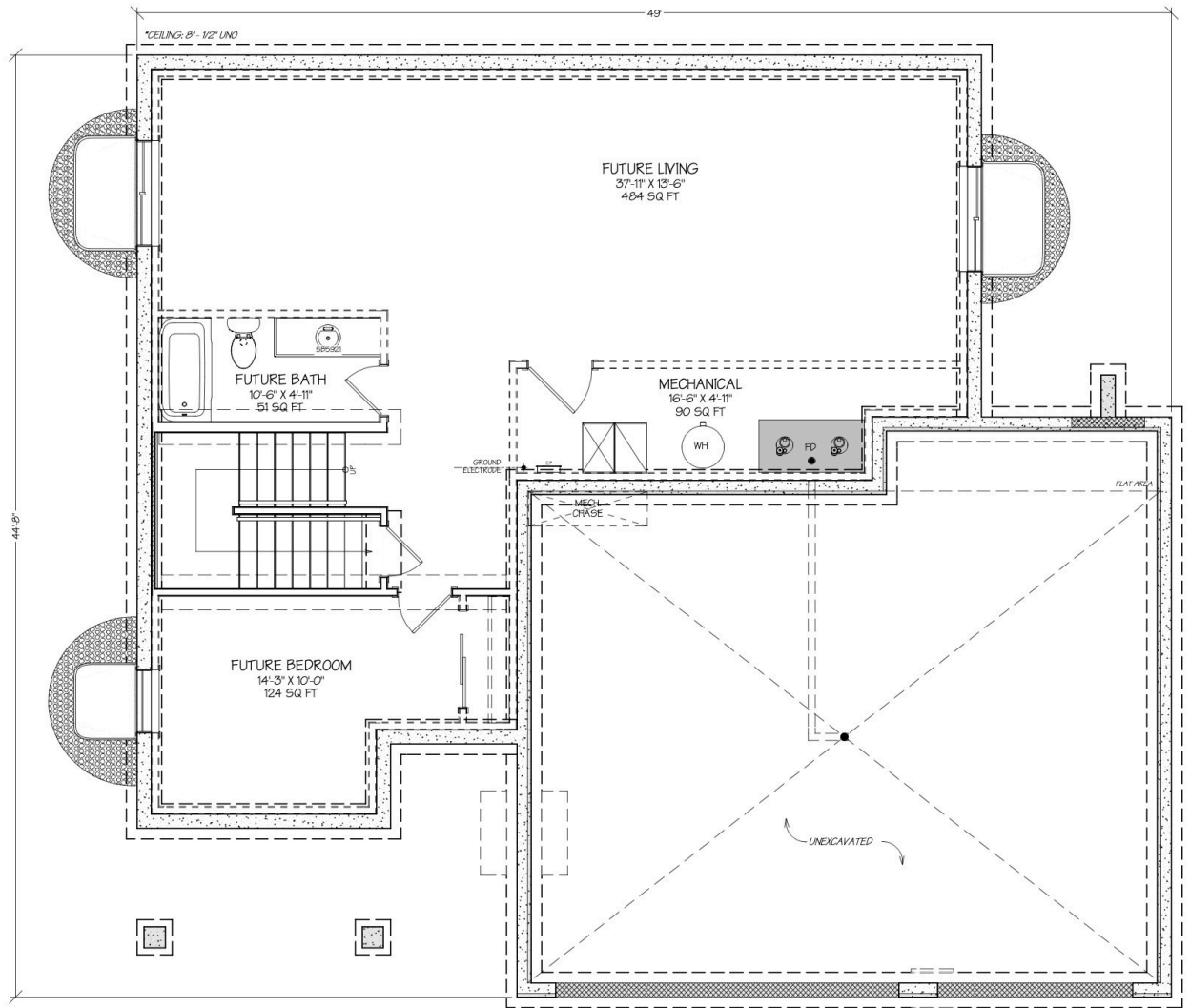
Augusta 3.0 - Base Plan - Lower Floor - 1,078 sq ft
