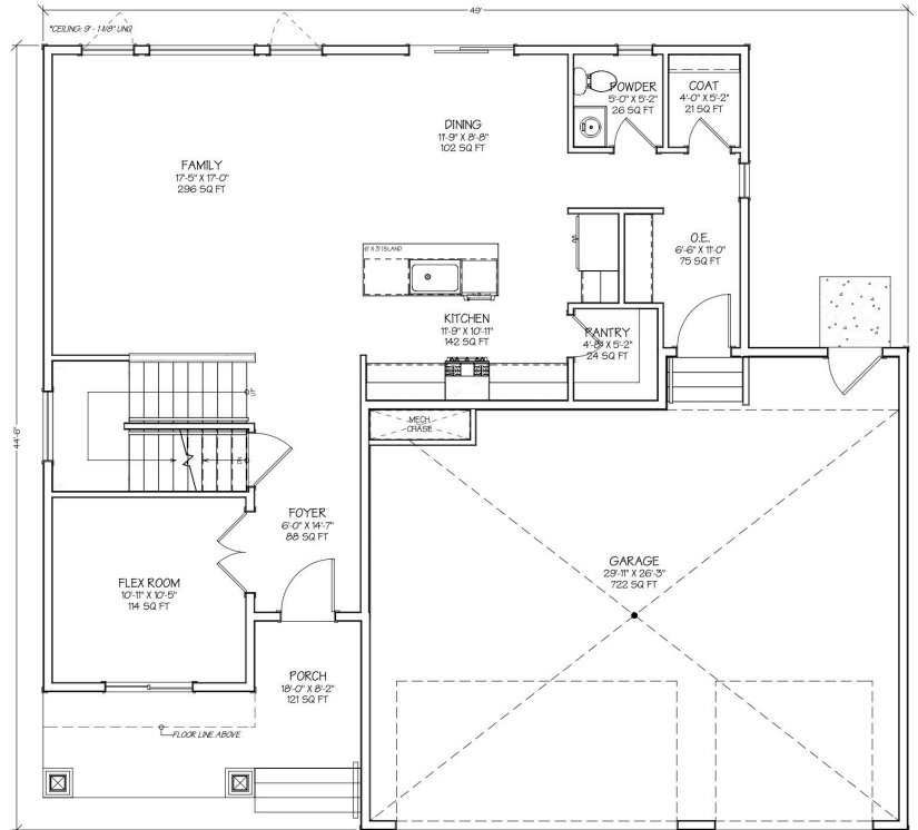
Augusta 3.0 - Base Plan - Main Floor - 1,078 sq ft
