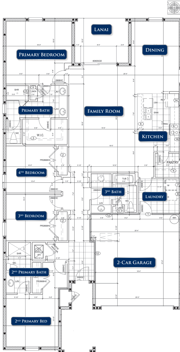
FLEX FLOOR PLAN
