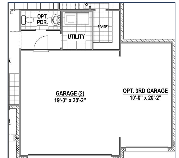
Optional 3rd Car Garage with Optional Powder Bath
