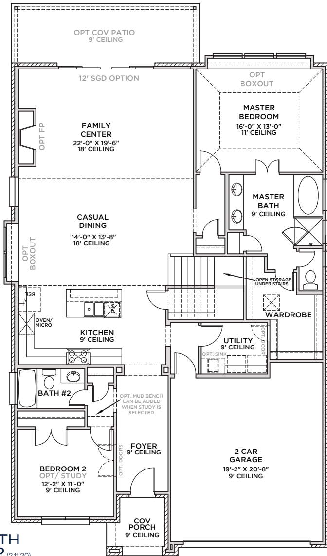
FIRST FLOOR
