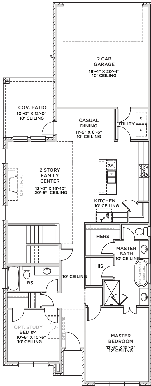
FIRST FLOOR
