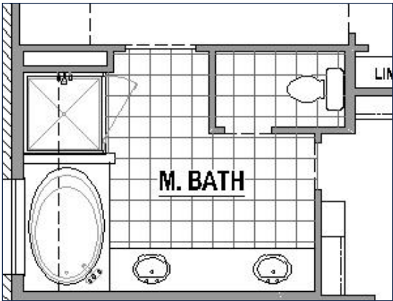
Optional Drop in Tub at Main Bath
