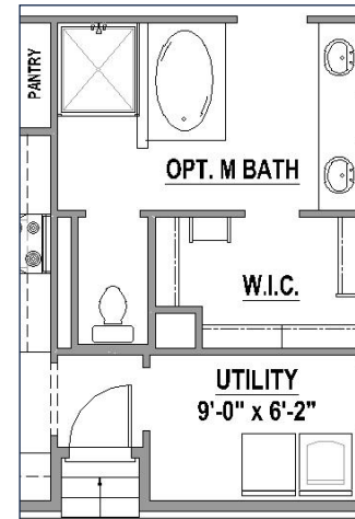
Alternate Main Bath Layout
