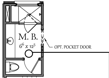
MASTER BATH LAYOUT- SUPER SHOWER OPTION
