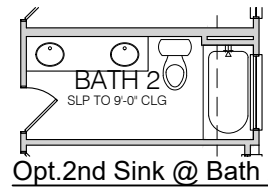
2nd Floor Plan
