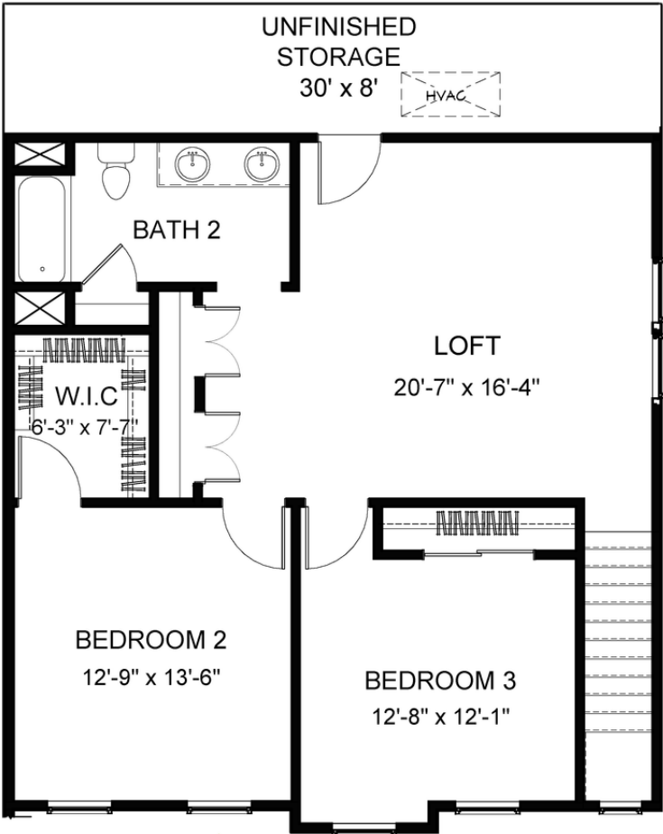
LOFT LEVEL
