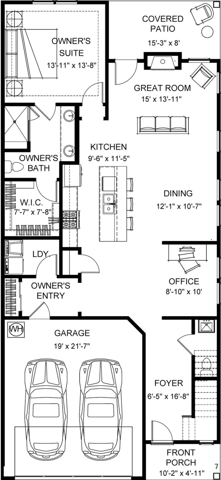
MAIN LEVEL
