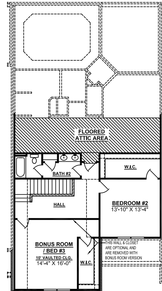
Second Floor
