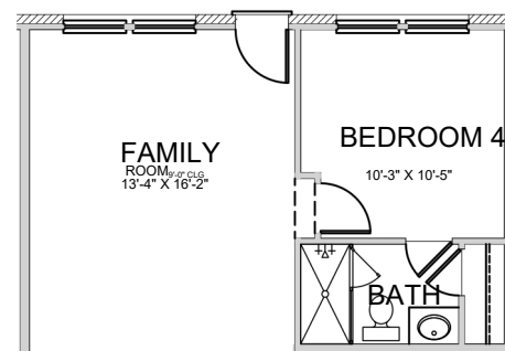
*Bedroom 4 Option ILO Study First Floor Plan
